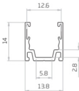
ST-23 Bendable Serrated Aluminium Mounting Profile
