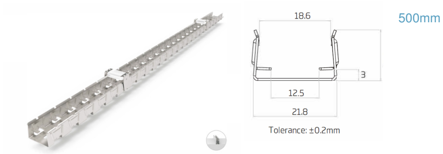
ST-2010 Stainless Steel Mounting Profile
